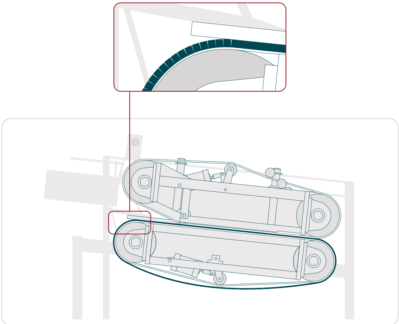
Continuous casting technology with dam blocks
